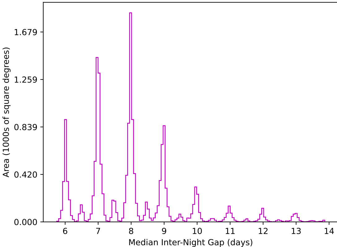
baseline_v3.3_10yrs WFD z band: Median Inter-Night Gap
