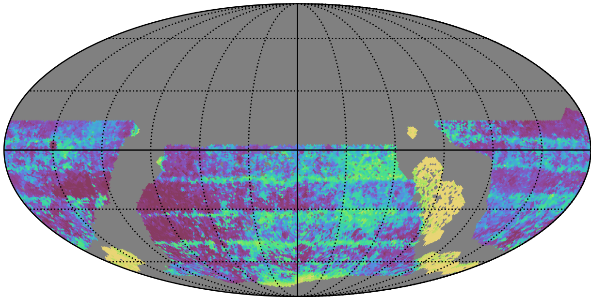
baseline_v3.3_10yrs WFD y band: Median Inter-Night Gap
