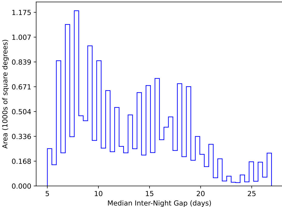
baseline_v3.3_10yrs WFD y band: Median Inter-Night Gap
