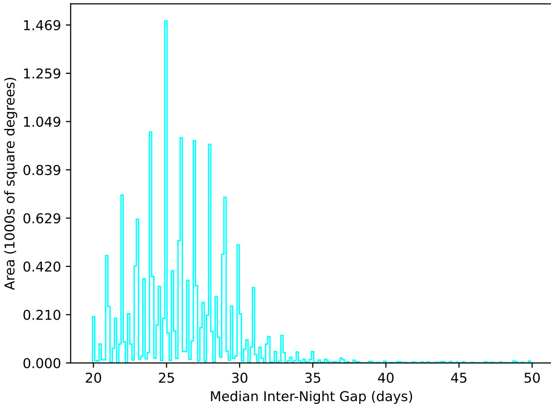
baseline_v3.3_10yrs WFD u band: Median Inter-Night Gap
