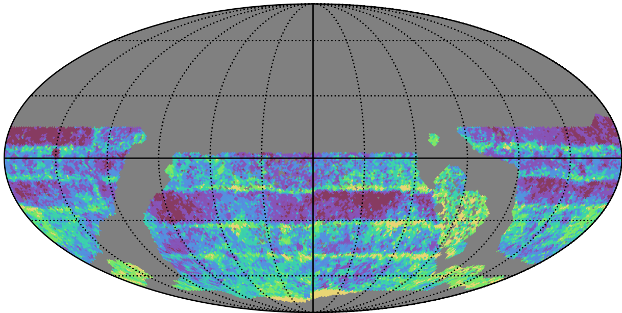
baseline_v3.3_10yrs WFD r band: Median Inter-Night Gap
