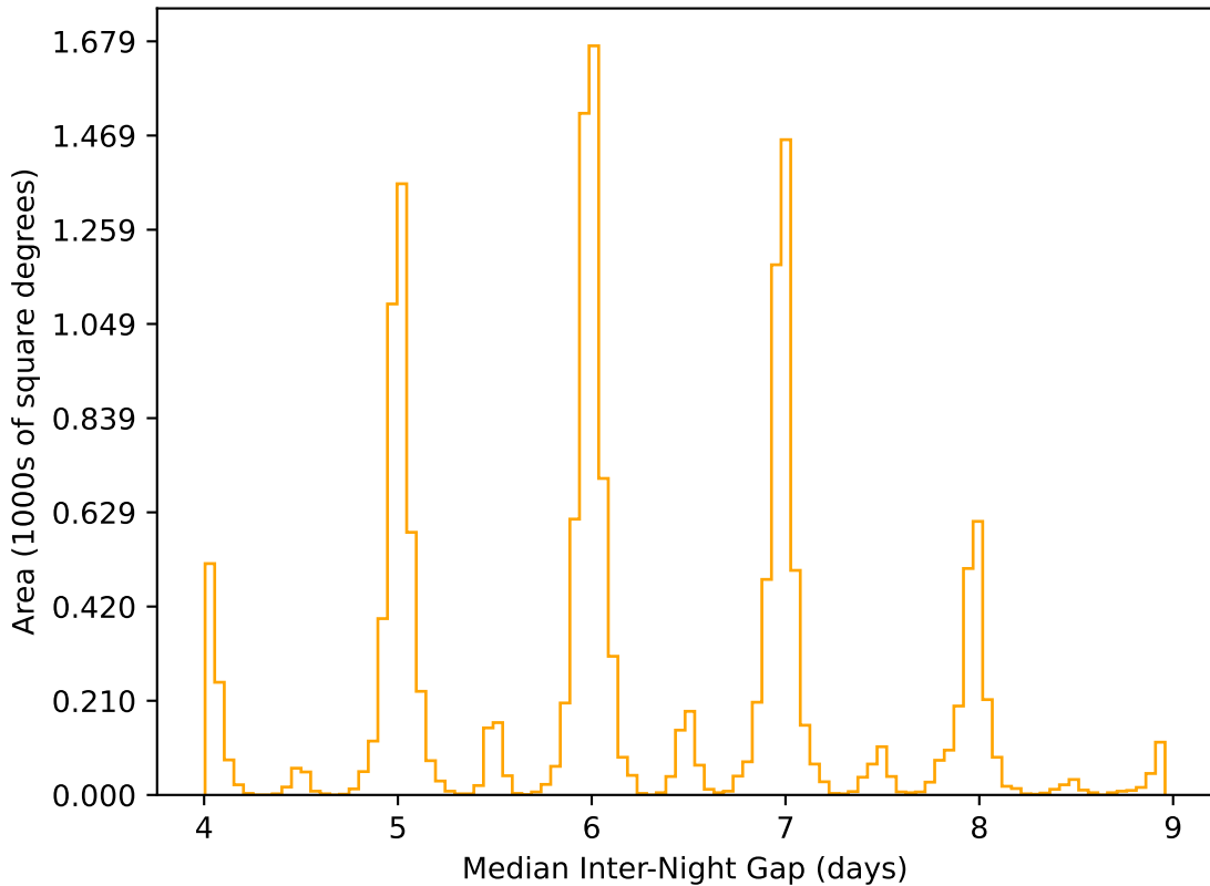
baseline_v3.3_10yrs WFD r band: Median Inter-Night Gap
