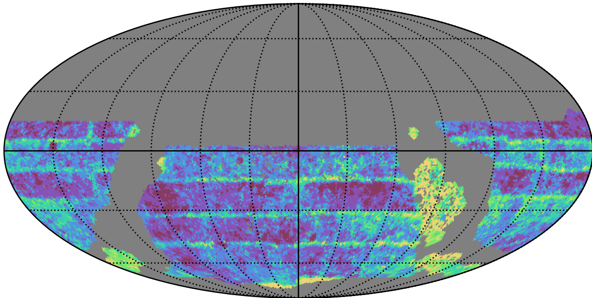
baseline_v3.3_10yrs WFD i band: Median Inter-Night Gap
