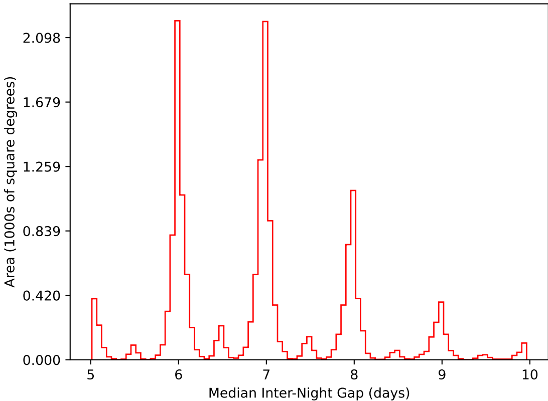
baseline_v3.3_10yrs WFD i band: Median Inter-Night Gap
