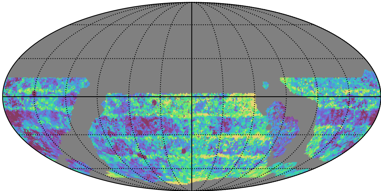
baseline_v3.3_10yrs WFD g band: Median Inter-Night Gap
