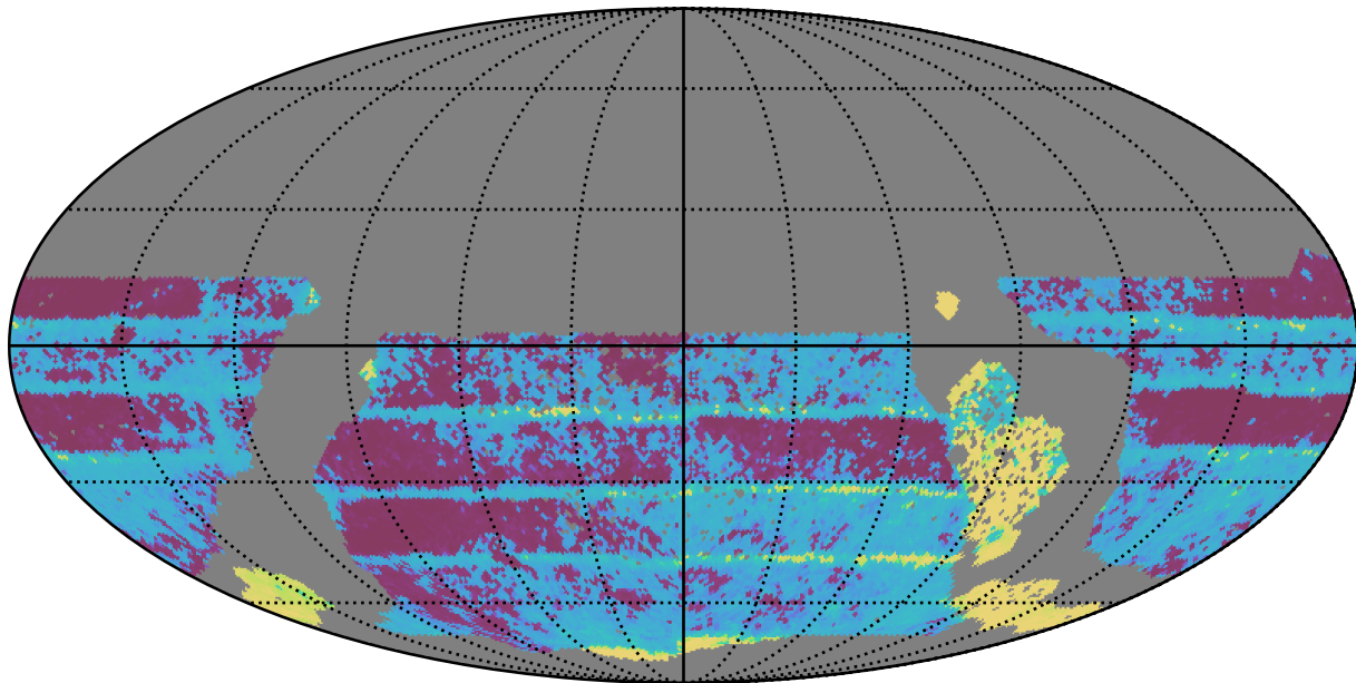
baseline_v3.3_10yrs WFD all bands: Median Inter-Night Gap
