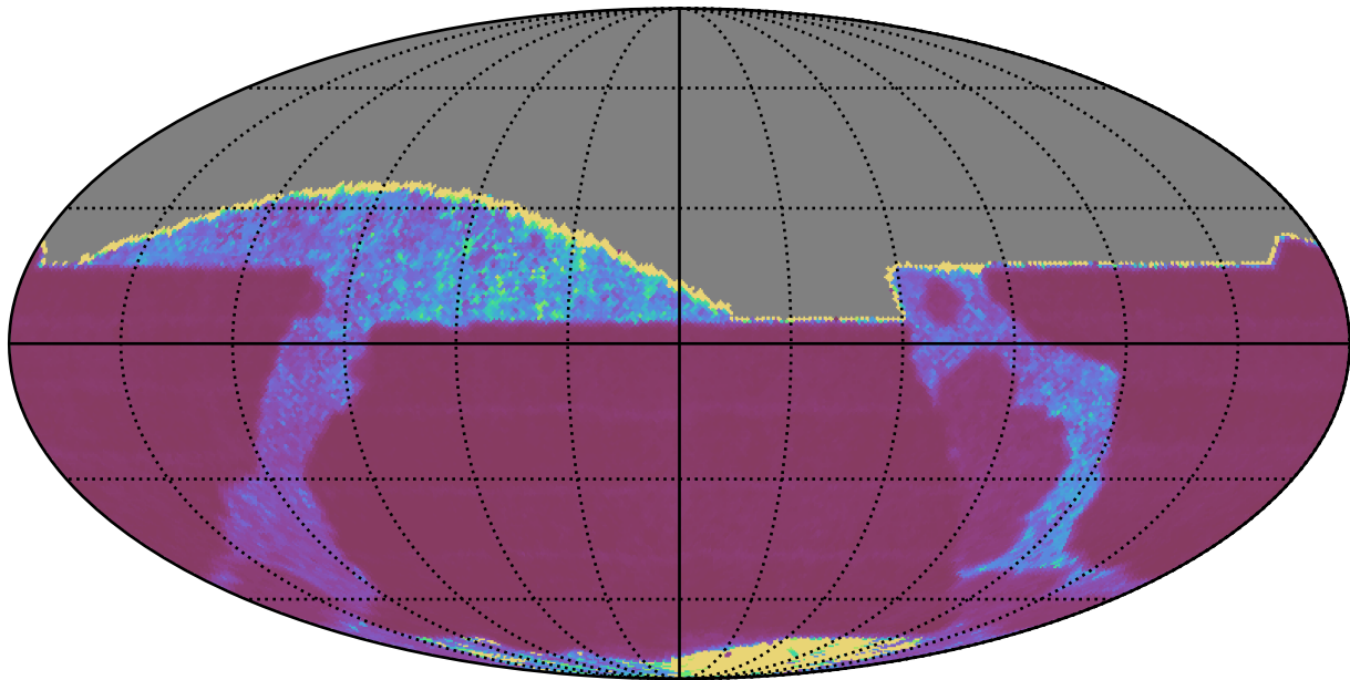
baseline_v3.3_10yrs All sky z band: Median Inter-Night Gap
