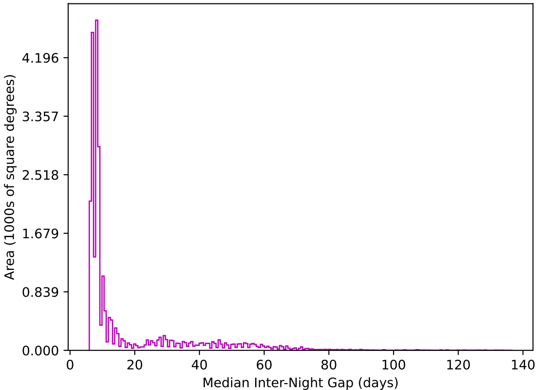
baseline_v3.3_10yrs All sky z band: Median Inter-Night Gap
