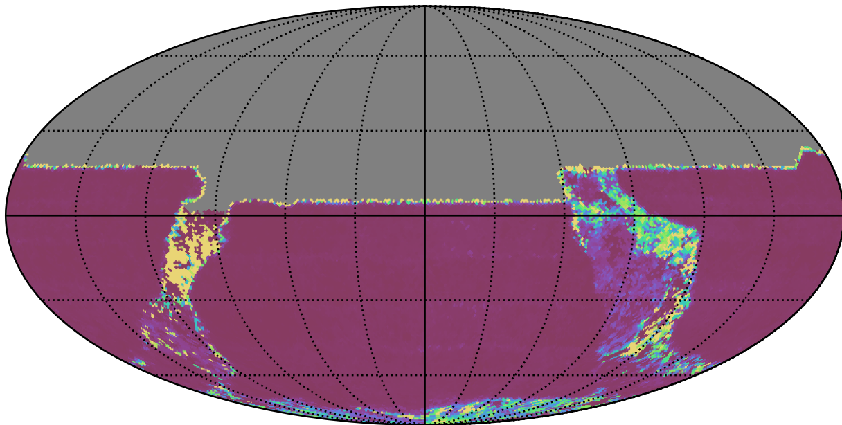
baseline_v3.3_10yrs All sky u band: Median Inter-Night Gap
