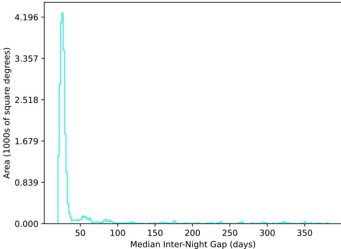
baseline_v3.3_10yrs All sky u band: Median Inter-Night Gap
