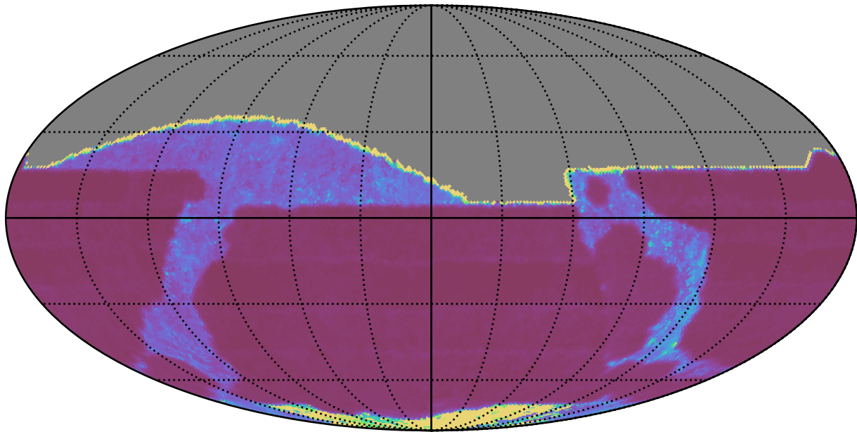
baseline_v3.3_10yrs All sky r band: Median Inter-Night Gap
