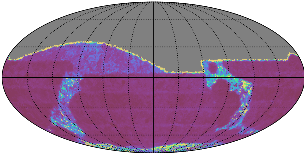
baseline_v3.3_10yrs All sky g band: Median Inter-Night Gap
