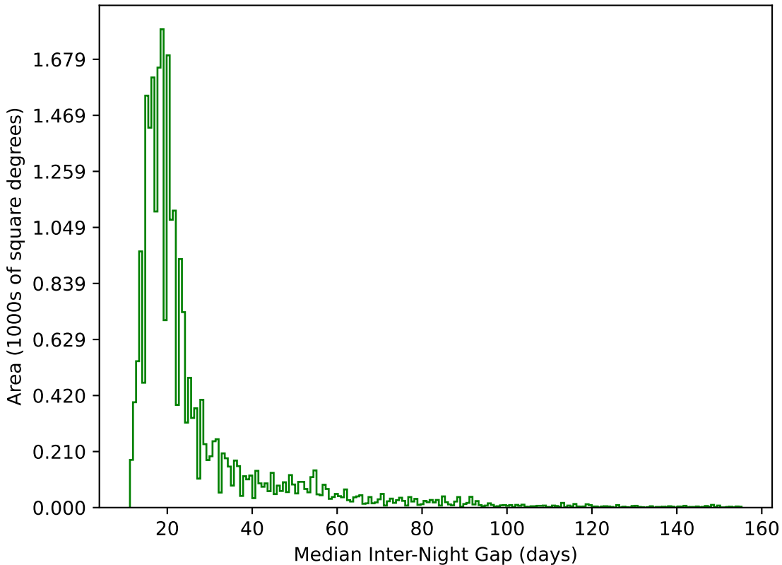
baseline_v3.3_10yrs All sky g band: Median Inter-Night Gap
