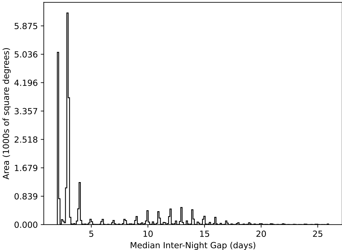
baseline_v3.3_10yrs All sky all bands: Median Inter-Night Gap
