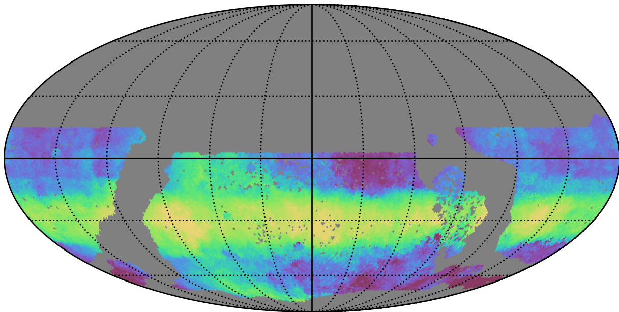
baseline_v3.3_10yrs WFD z band: Median HA
