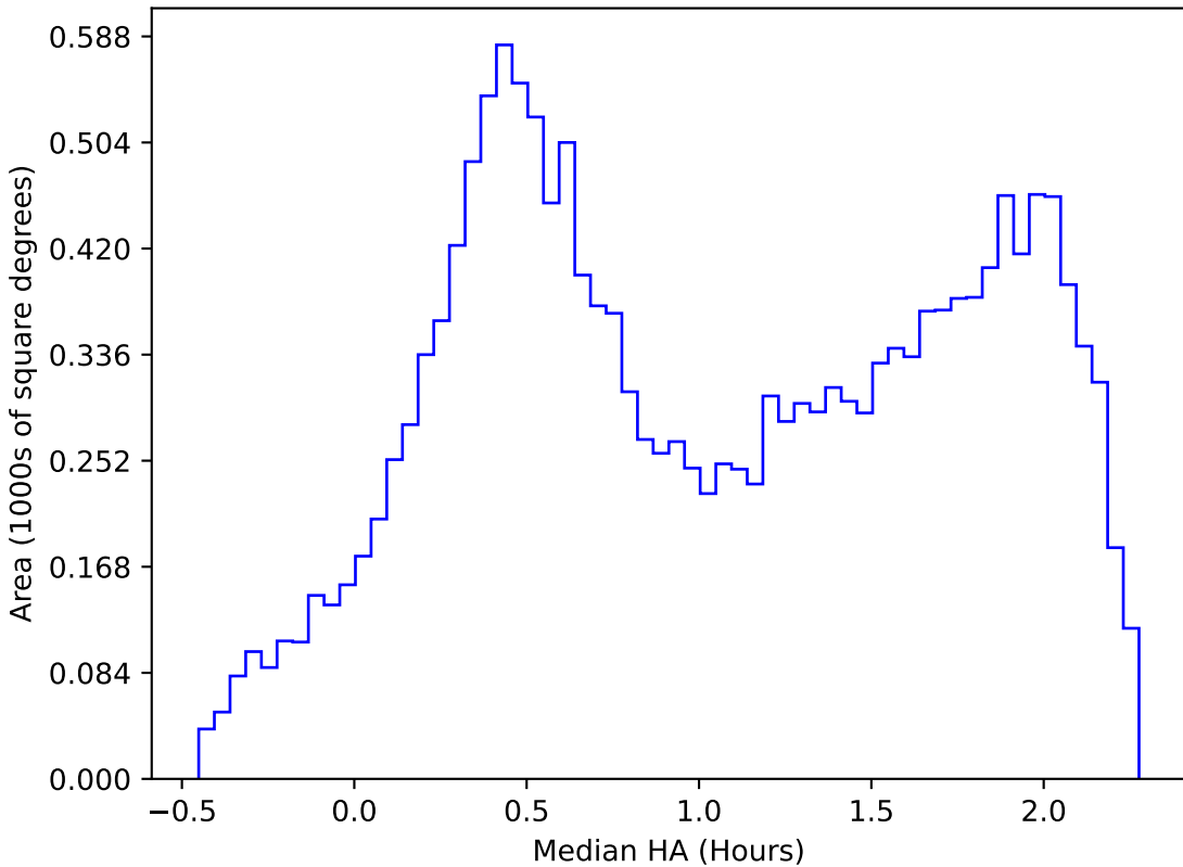
baseline_v3.3_10yrs WFD z band: Median HA
