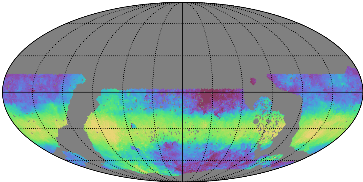
baseline_v3.3_10yrs WFD y band: Median HA
