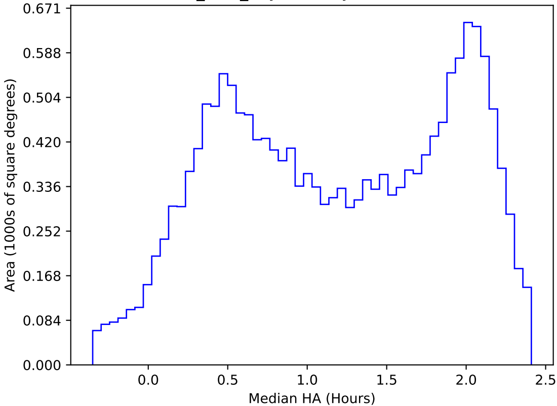
baseline_v3.3_10yrs WFD y band: Median HA
