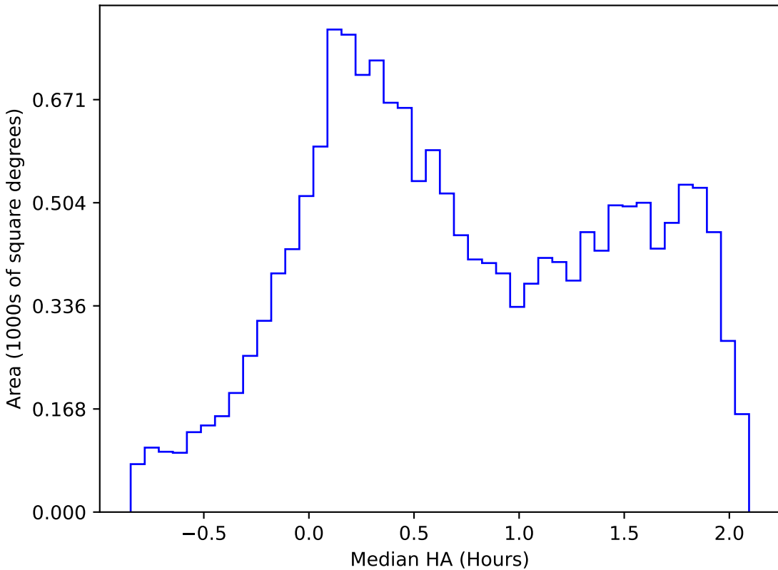
baseline_v3.3_10yrs WFD r band: Median HA
