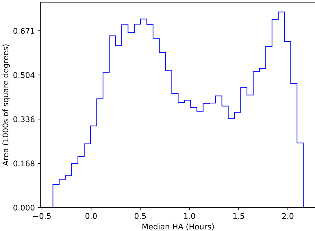
baseline_v3.3_10yrs WFD i band: Median HA
