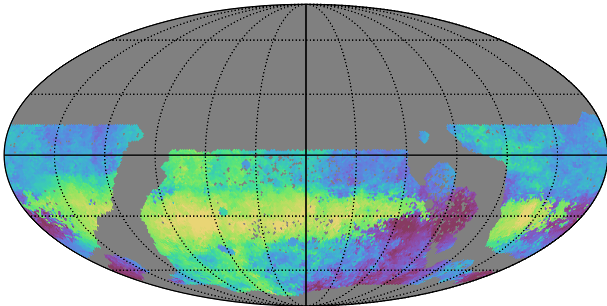
baseline_v3.3_10yrs WFD g band: Median HA
