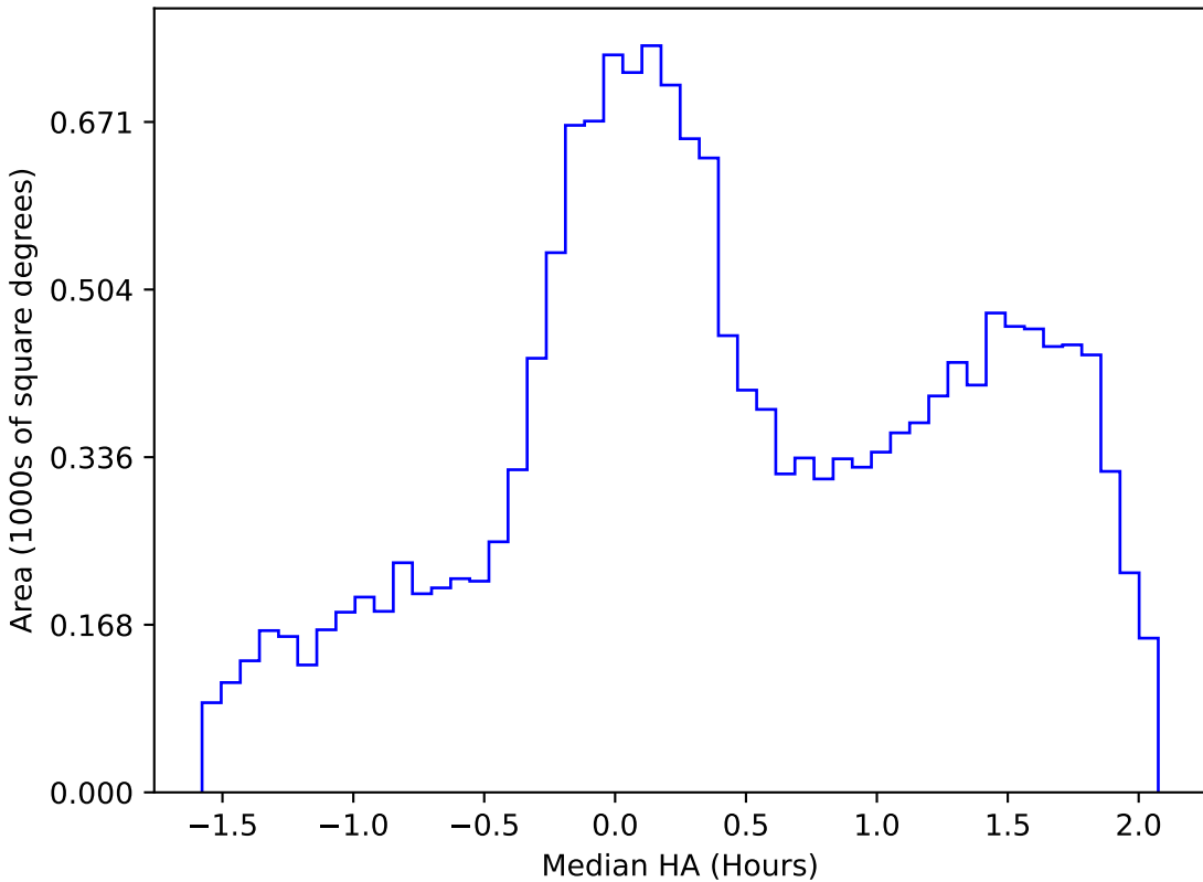
baseline_v3.3_10yrs WFD g band: Median HA
