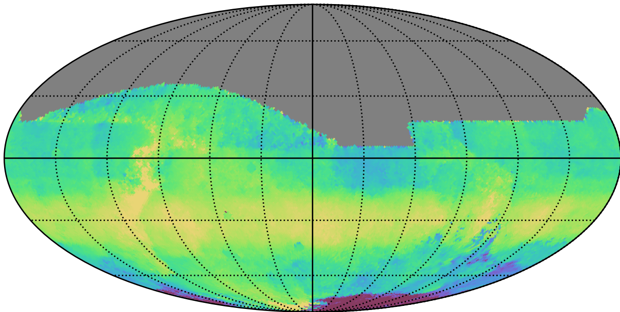
baseline_v3.3_10yrs All sky z band: Median HA
