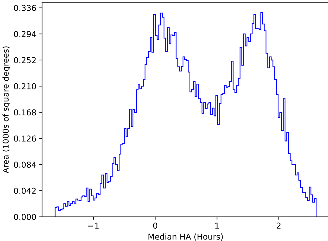
baseline_v3.3_10yrs All sky u band: Median HA
