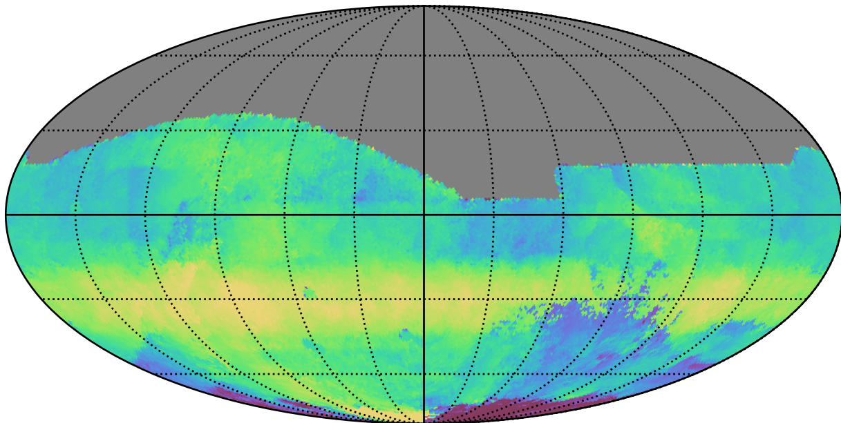
baseline_v3.3_10yrs All sky r band: Median HA
