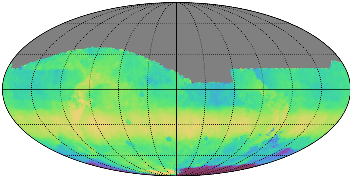
baseline_v3.3_10yrs All sky i band: Median HA
