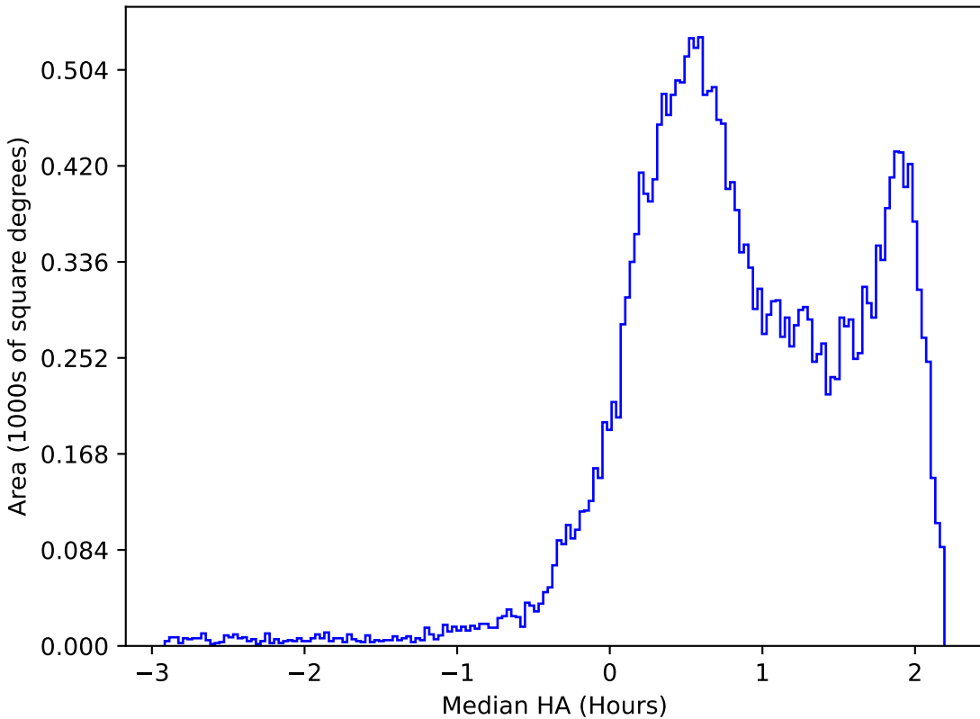
baseline_v3.3_10yrs All sky i band: Median HA
