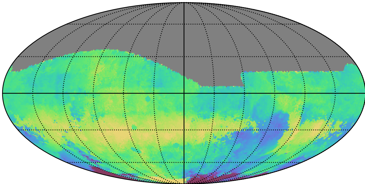
baseline_v3.3_10yrs All sky g band: Median HA
