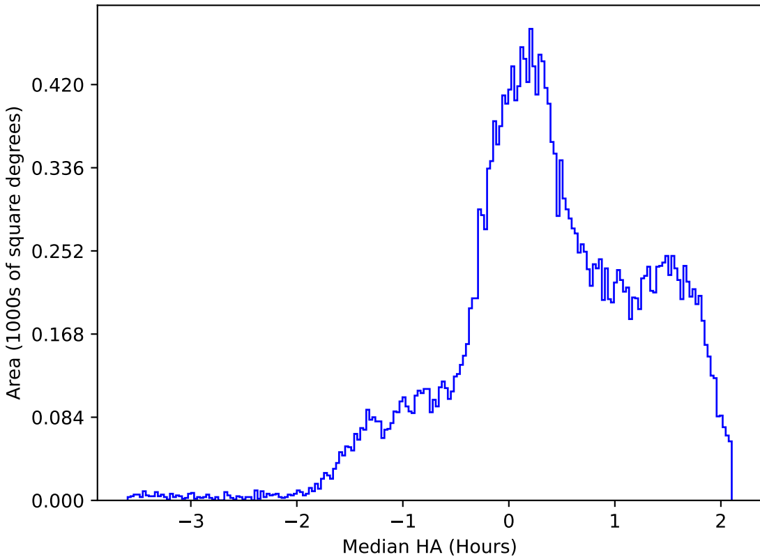
baseline_v3.3_10yrs All sky g band: Median HA
