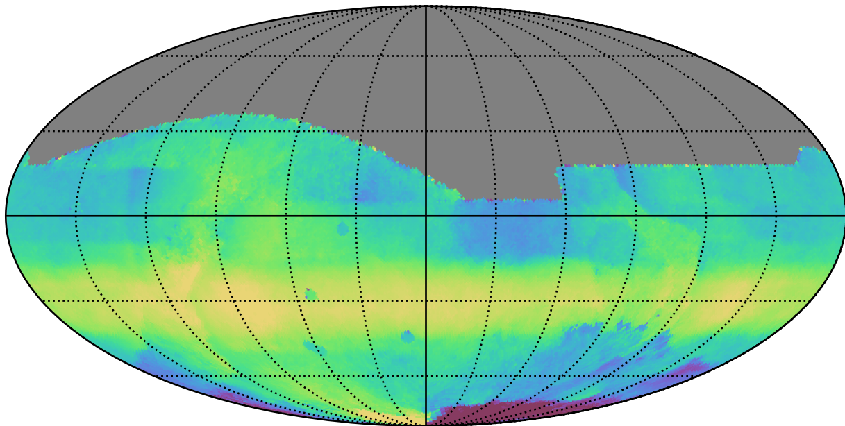
baseline_v3.3_10yrs All sky all bands: Median HA
