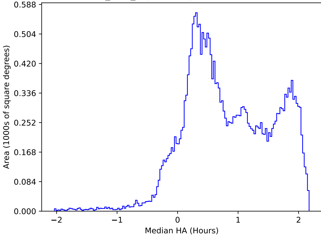
baseline_v3.3_10yrs All sky all bands: Median HA
