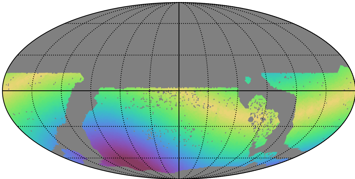
baseline_v3.3_10yrs WFD u band: Max solarElong
