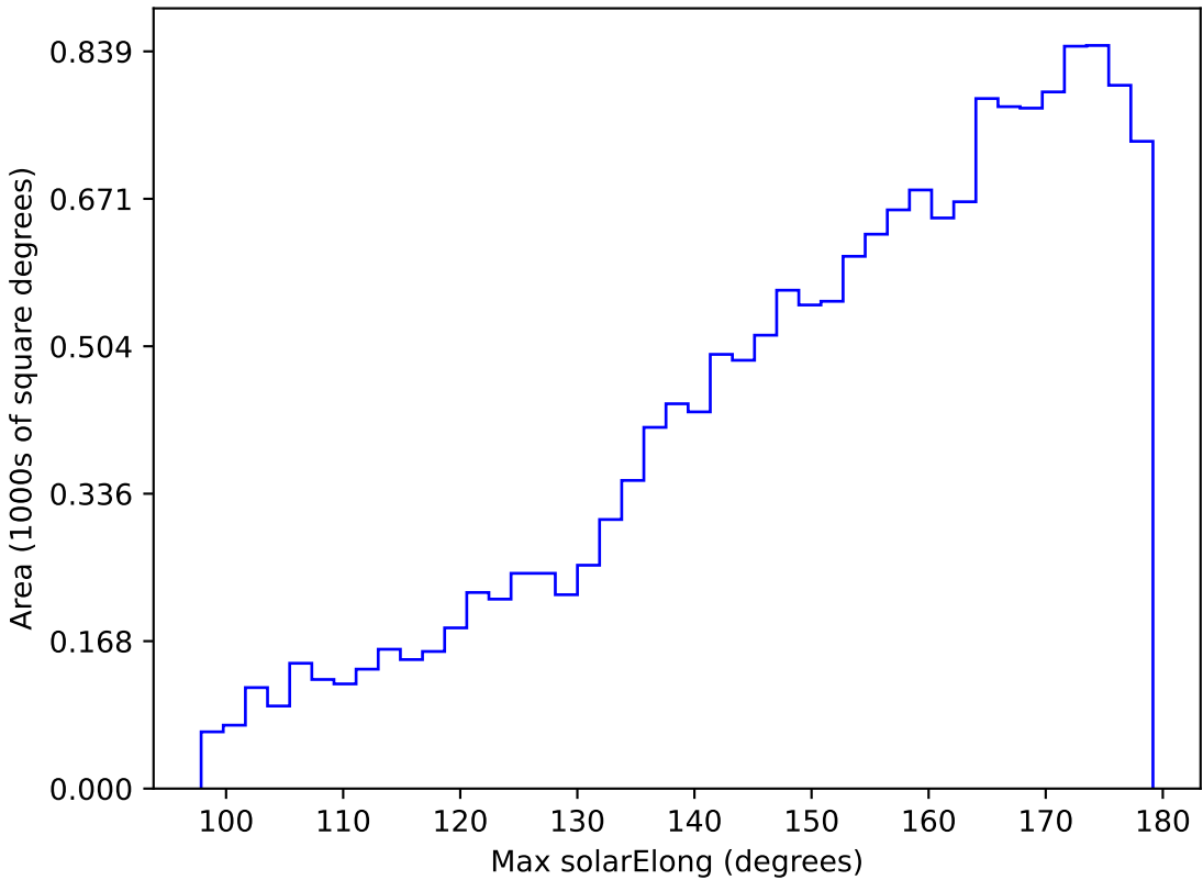
baseline_v3.3_10yrs WFD u band: Max solarElong
