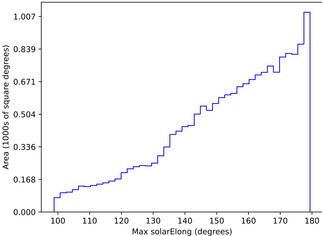
baseline_v3.3_10yrs WFD r band: Max solarElong
