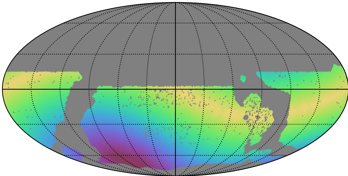
baseline_v3.3_10yrs WFD g band: Max solarElong
