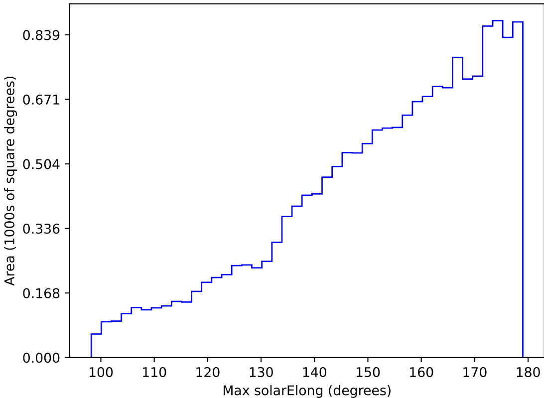
baseline_v3.3_10yrs WFD g band: Max solarElong
