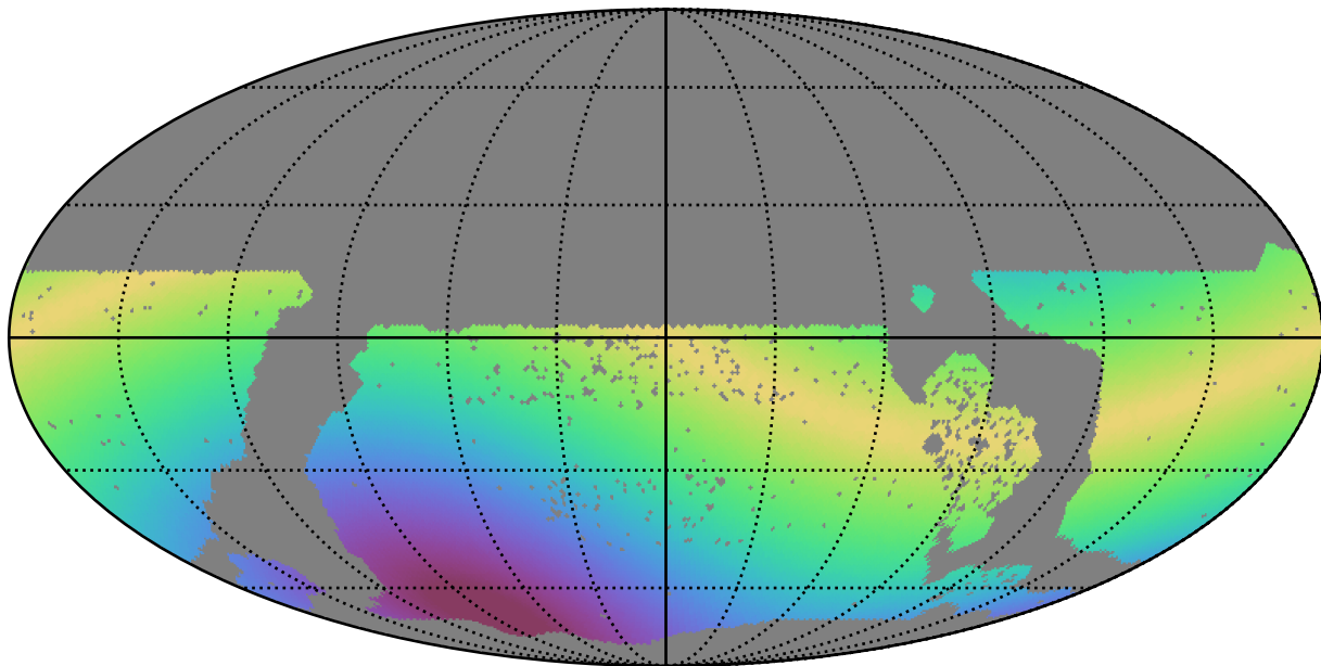
baseline_v3.3_10yrs WFD all bands: Max solarElong
