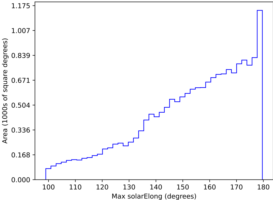
baseline_v3.3_10yrs WFD all bands: Max solarElong
