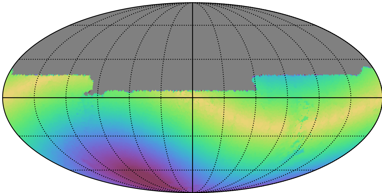
baseline_v3.3_10yrs All sky u band: Max solarElong
