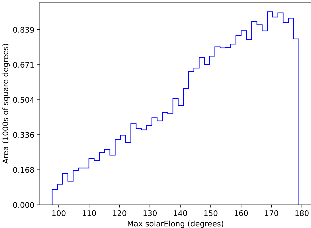
baseline_v3.3_10yrs All sky u band: Max solarElong
