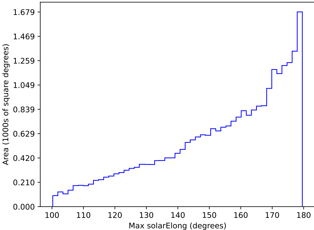
baseline_v3.3_10yrs All sky all bands: Max solarElong
