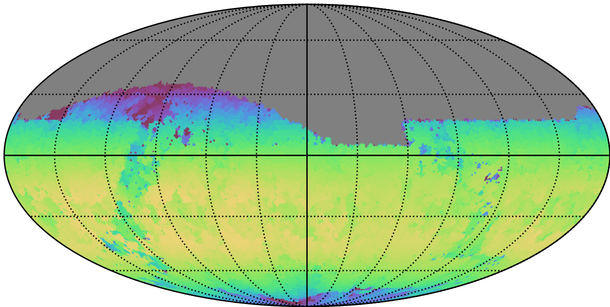
baseline_v3.3_10yrs Yr 1 z band: Max skyBrightness
