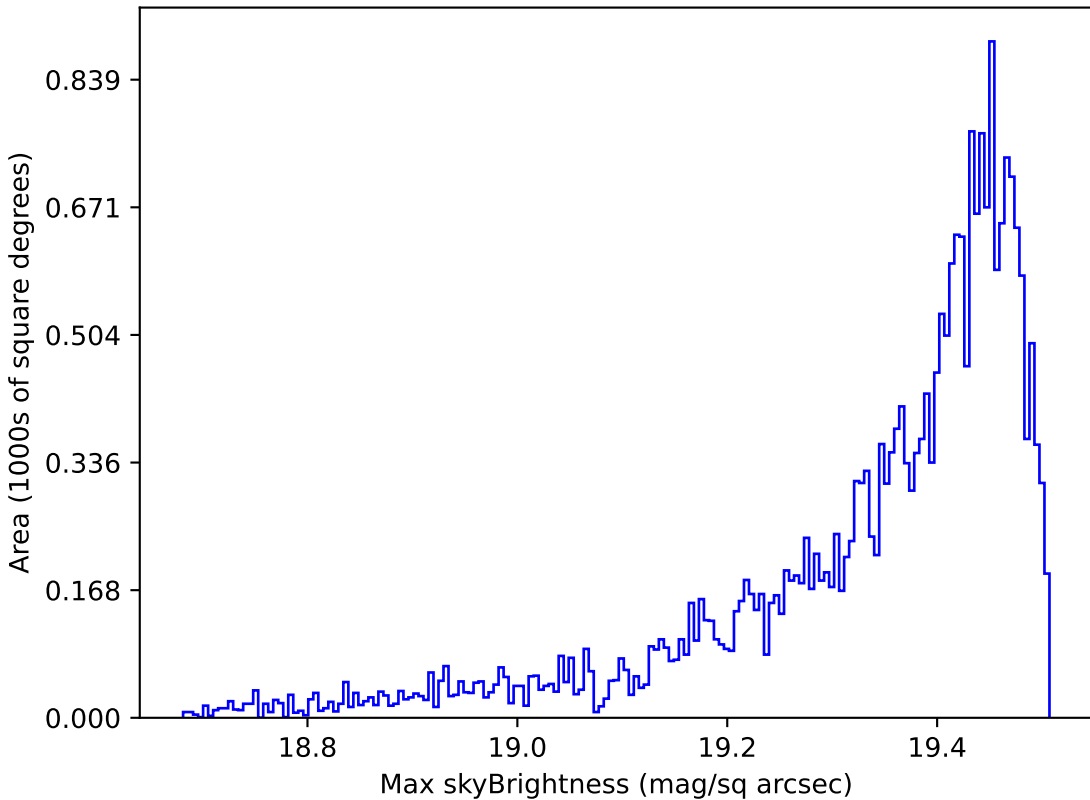
baseline_v3.3_10yrs Yr 1 z band: Max skyBrightness
