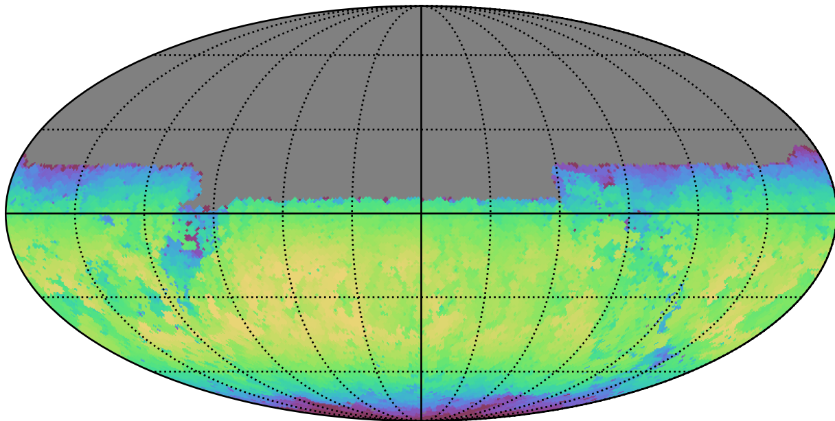
baseline_v3.3_10yrs Yr 1 y band: Max skyBrightness
