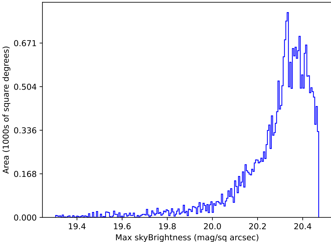
baseline_v3.3_10yrs Yr 1 i band: Max skyBrightness
