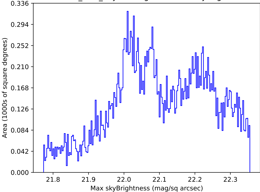
baseline_v3.3_10yrs Yr 1 g band: Max skyBrightness
